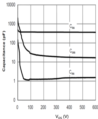
Figure 8: Capacitance Characteristics
