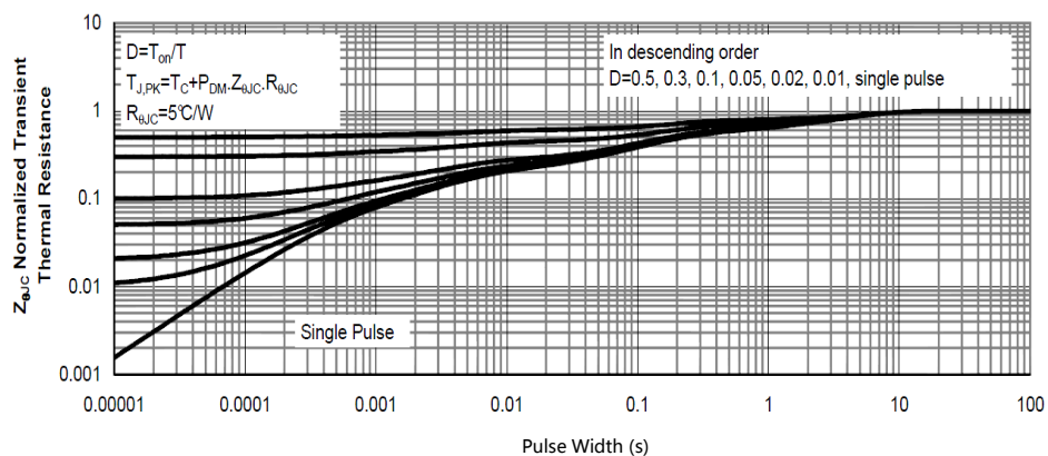
Figure 15: Normalized Maximum Transient Thermal Impedance
