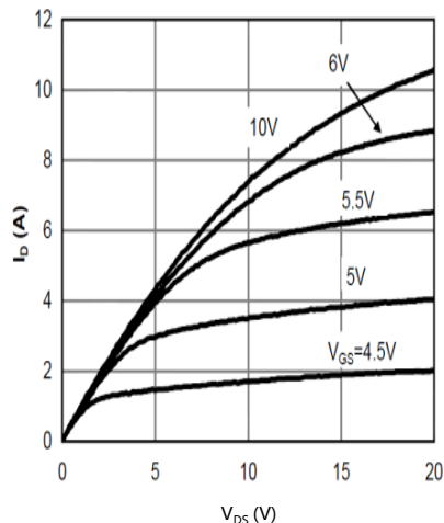
Figure 2: On-Region Characteristics@125°C
