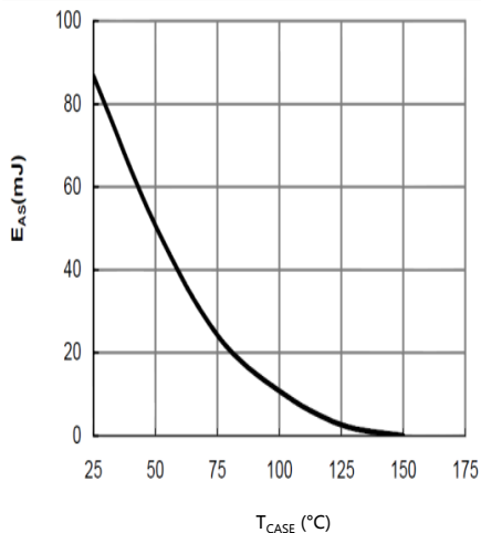
Figure 11: Avalanche energy
