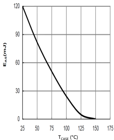
Figure 11: Avalanche energy
