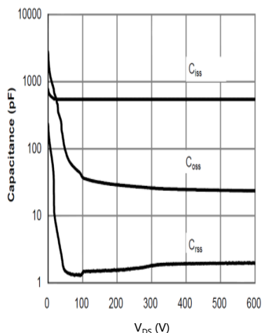
Figure 8: Capacitance Characteristics
