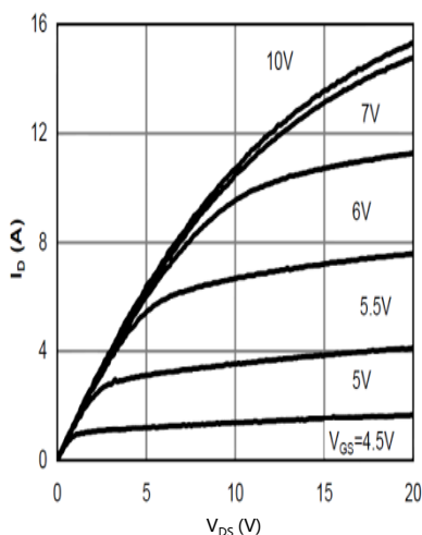
Figure 2: On-Region Characteristics@125°C
