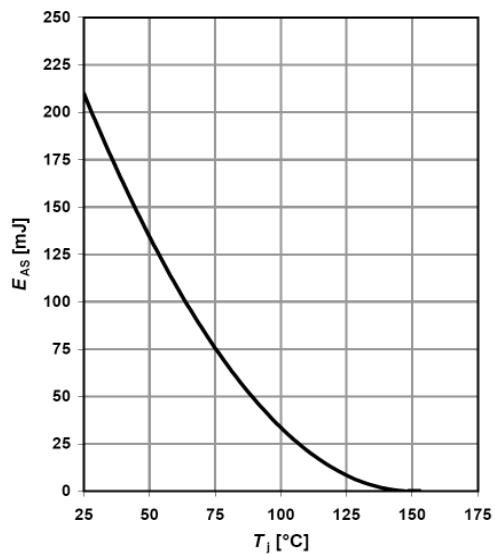
Avalanche energy
