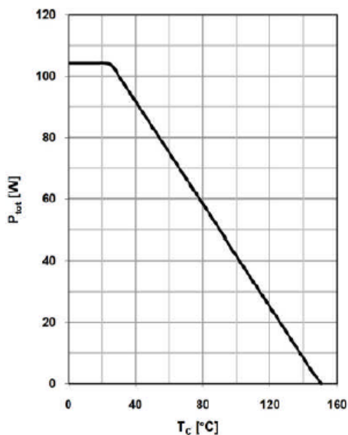
Power dissipation
