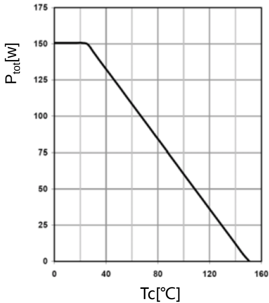
Power dissipation
