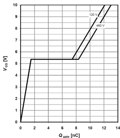
Figure 7: Gate-Charge Characteristics
