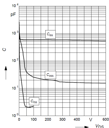
Figure 8: Capacitance Characteristics
