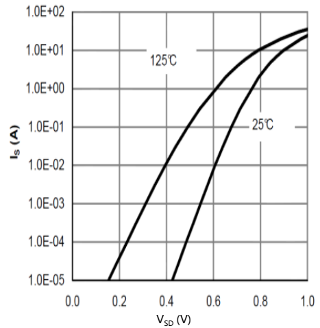
Figure 6: Body-Diode Characteristics
