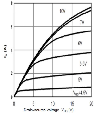
Figure 2: On-Region Characteristics@125°C
