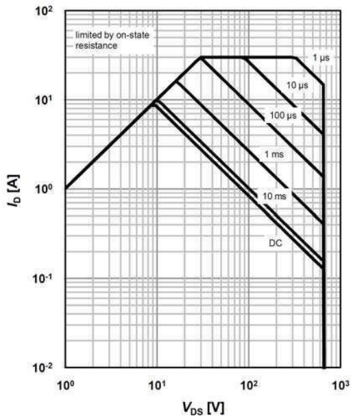
Safe operating area T_c = 25\text{ °C}
