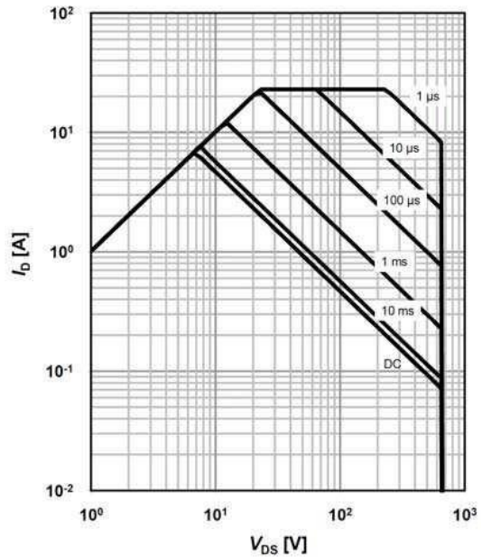
Safe operating area T_c = 80\text{ °C}
