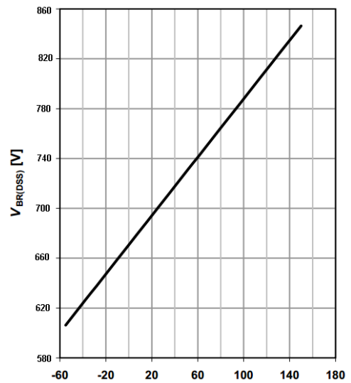
Drain-source breakdown voltage
