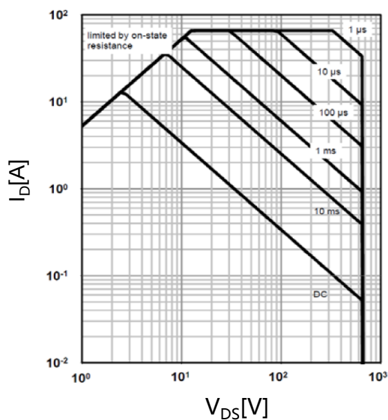
Safe operating area T_c=25\text{ °C}
