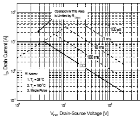
Figure 9-2. Maximum Safe Operating Area for TSF630M
