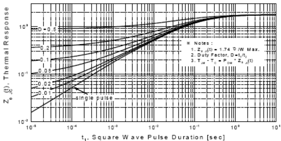
Figure 11-1. Transient Thermal Response Curve for TSP630M
