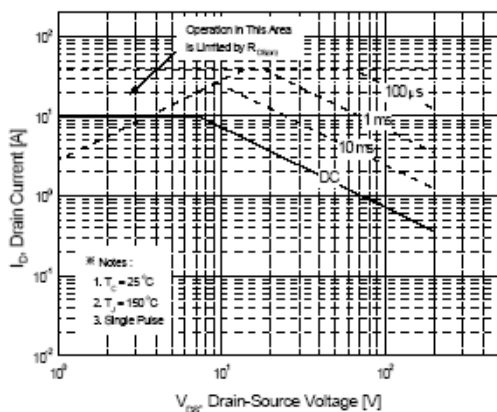
Figure 9-1. Maximum Safe Operating Area for TSP630M
