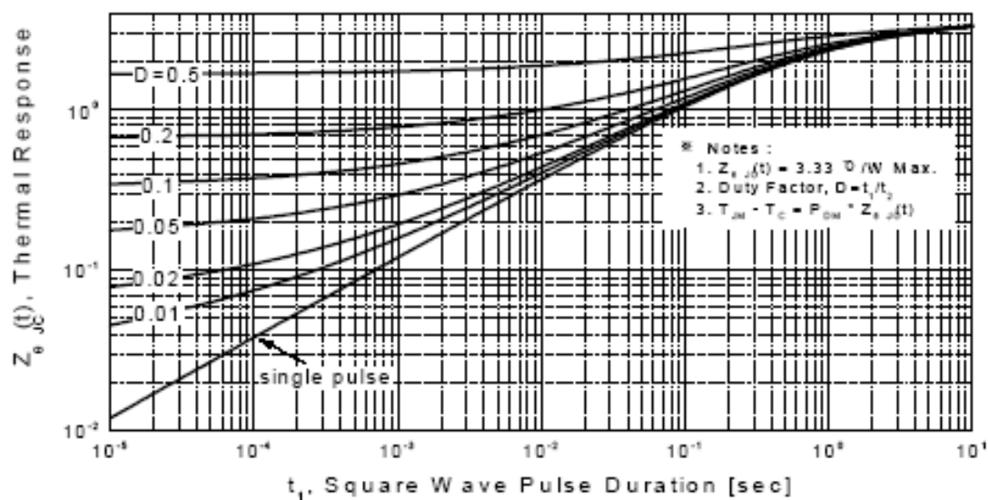
Figure 11-2. Transient Thermal Response Curve for TSF630M
