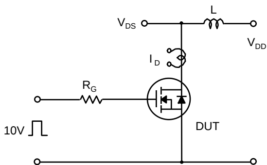
Fig 13. Unclamped Inductive Switching Test Circuit &amp; Waveforms
