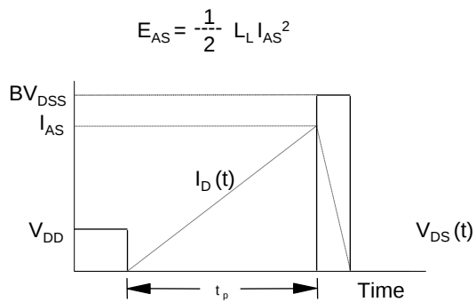
Fig 13. Unclamped Inductive Switching Test Circuit &amp; Waveforms
