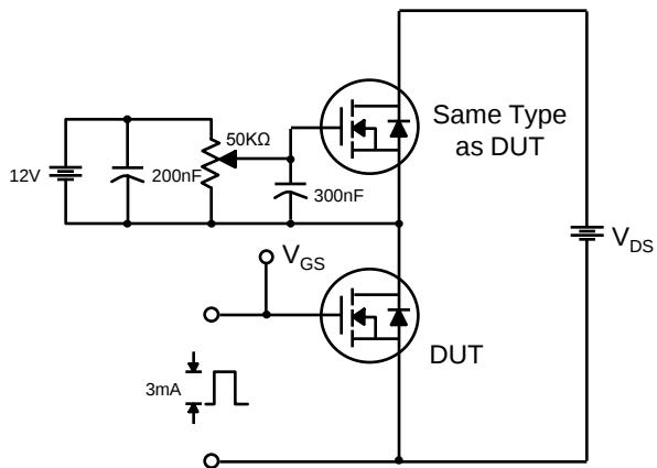
Fig 11. Gate Charge Test Circuit &amp; Waveform
