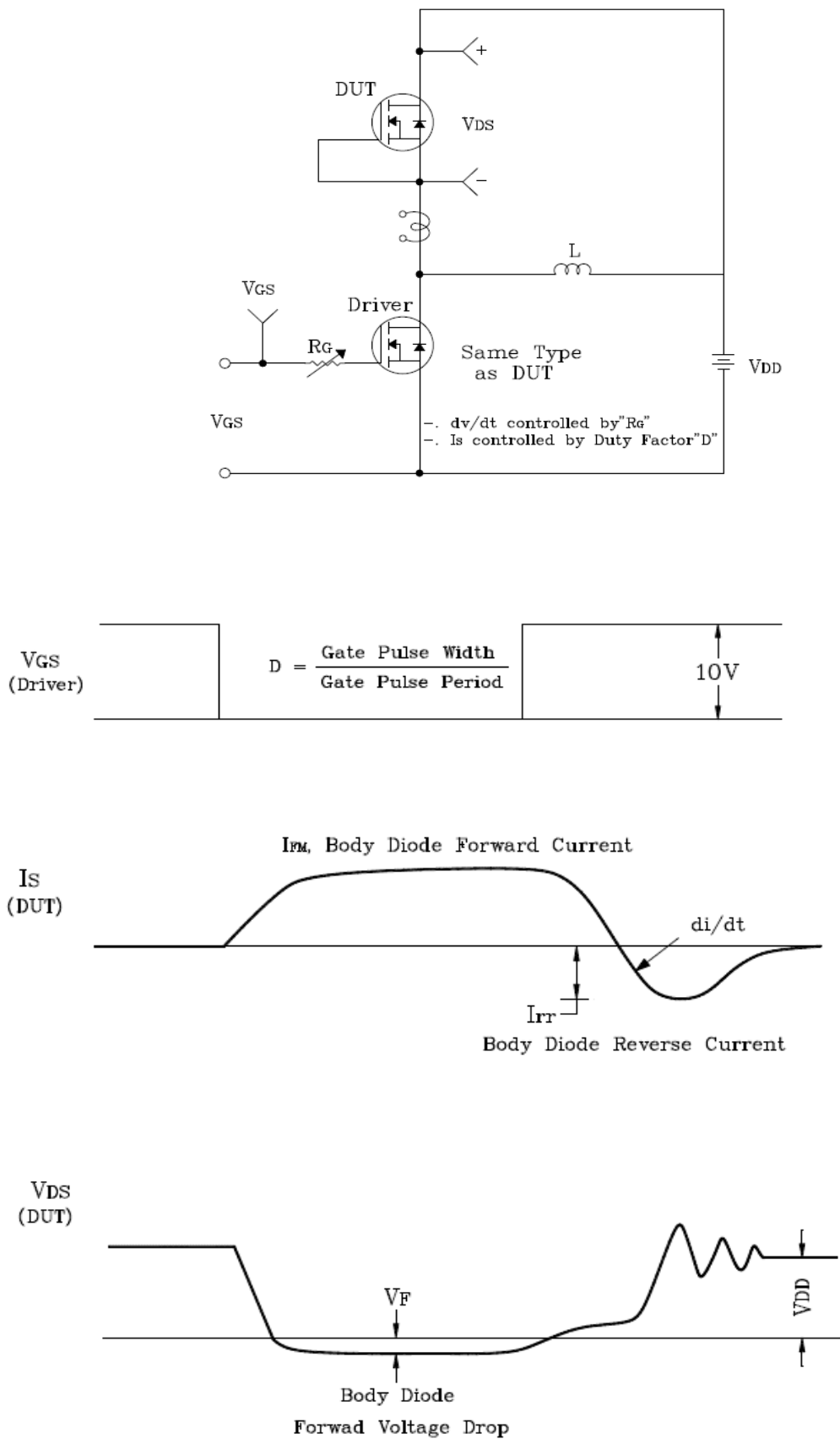
Fig. 15 Diode Reverse Recovery Time Test Circuit & Waveform
