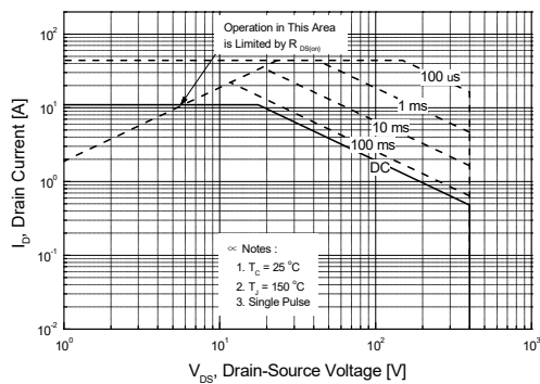
Figure 9-1. Maximum Safe Operating Area for TSP740MR
