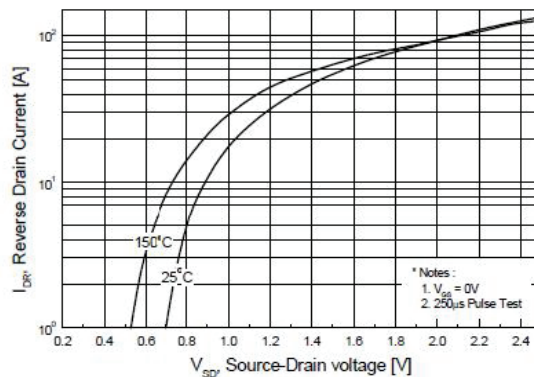
Figure 4. Body Diode Forward Voltage
