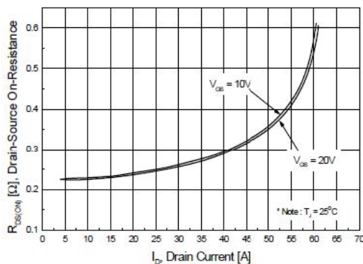
Figure 3. On-Resistance Variation
