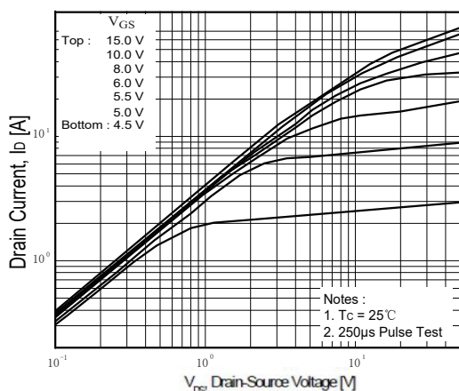
Figure 1. On-Region Characteristics
