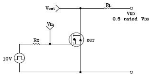
Fig. 13 Resistive Switching Test Circuit & Waveform
