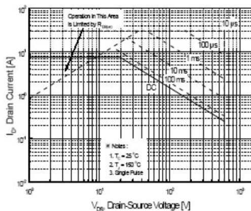
Figure 9-1. Maximum Safe Operating Area for TSP7N60M
