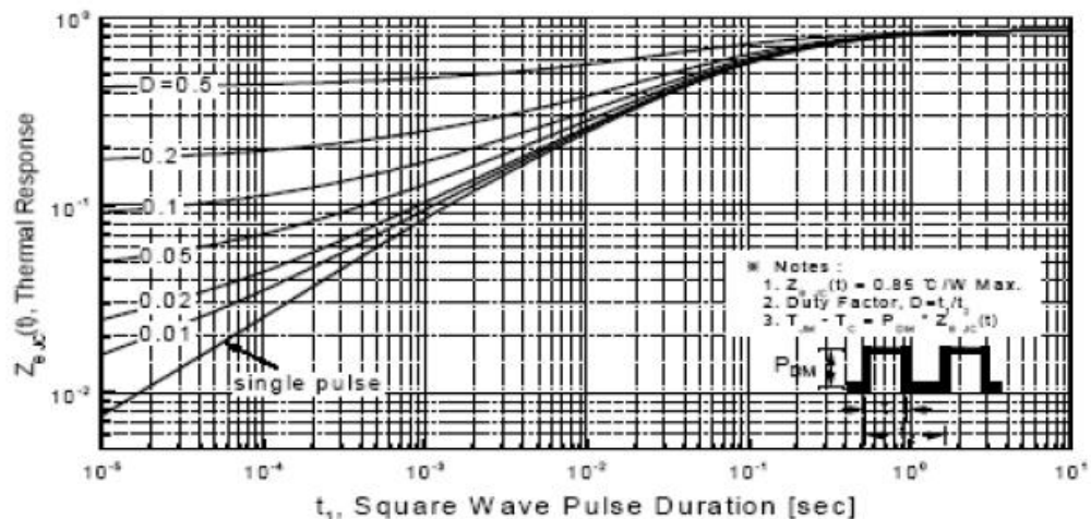
Figure 11-1. Transient Thermal Response Curve for TSP7N60M
