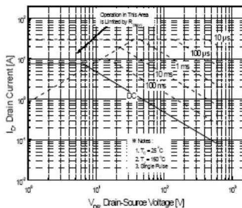
Figure 9-2. Maximum Safe Operating Area for TSF7N60M
