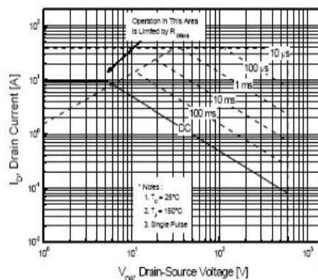
Figure 9-2. Maximum Safe Operating Area for TSF10N60M
