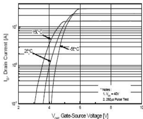
Figure 2. Transfer Characteristics
