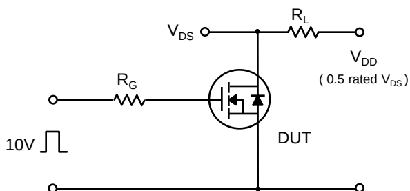
Fig 13. Resistive Switching Test Circuit & Waveforms
