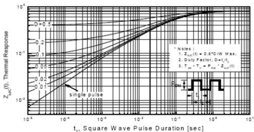
Figure 11-1. Transient Thermal Response Curve for TSP10N65M
