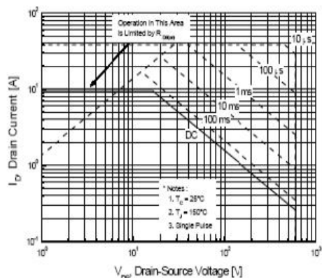
Figure 9-1. Maximum Safe Operating Area for TSP10N65M
