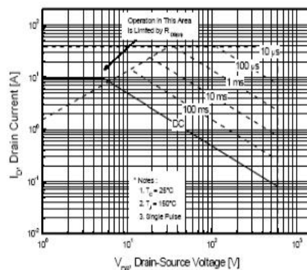
Figure 9-2. Maximum Safe Operating Area for TSF10N65M
