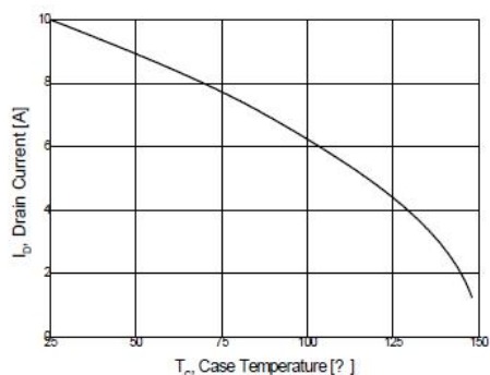
Figure 10. Maximum Drain Current vs Case Temperature
